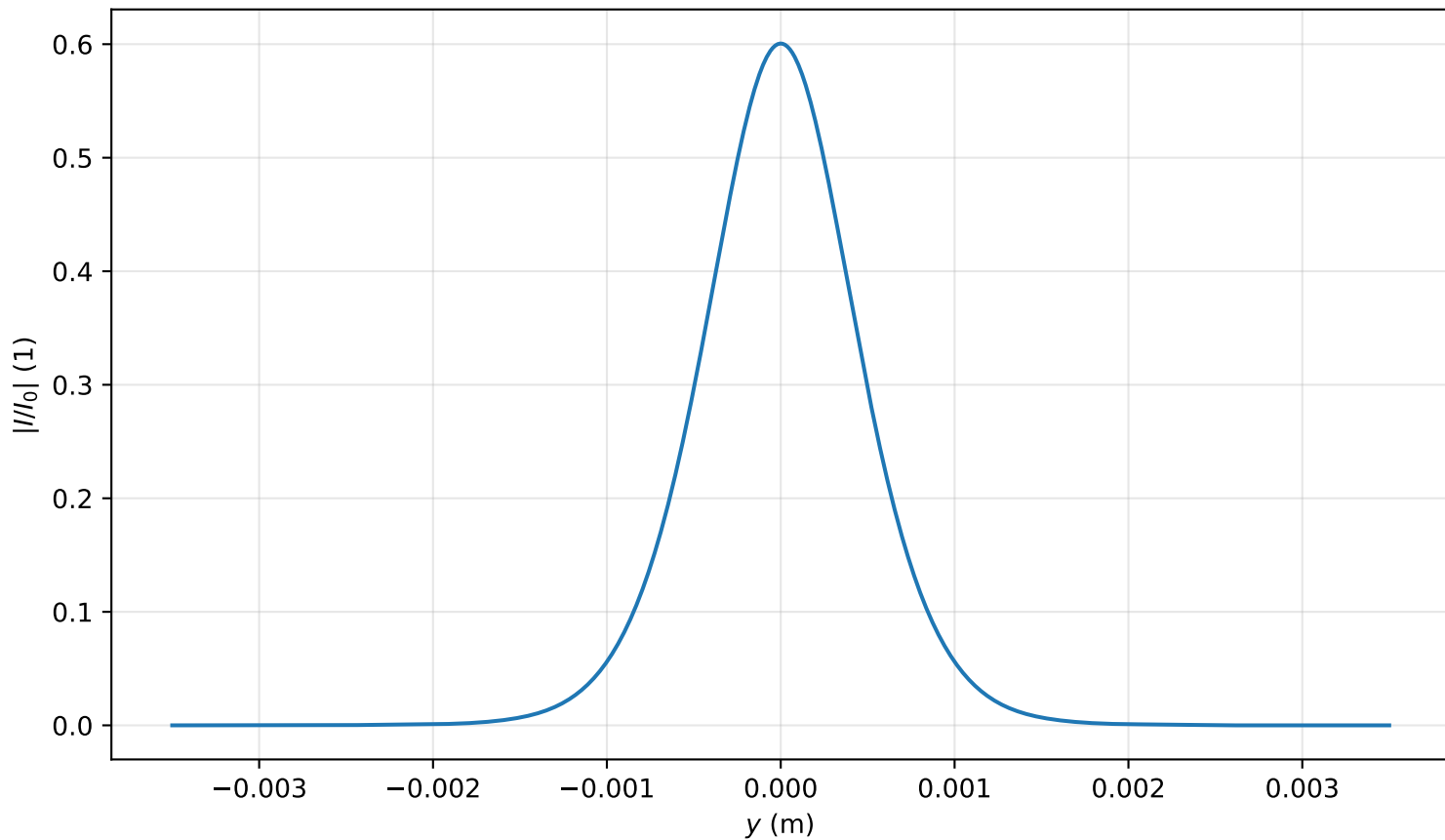
Intensity profile I(x = 0, y, z = 3.344)/I_0 , P_{in}=0.6P_{cr} , artificial time
